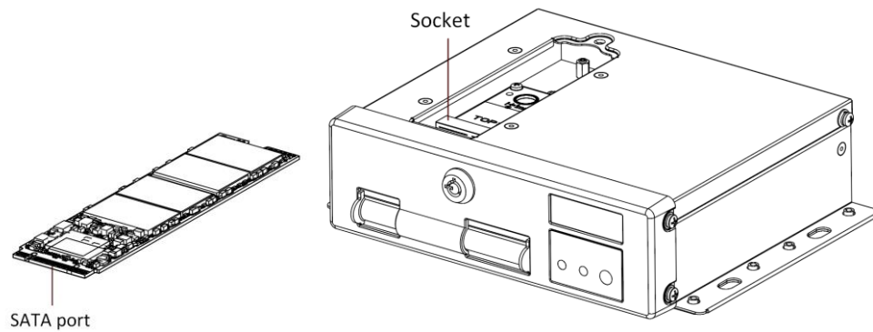
Figure 2-13 Install SSD
