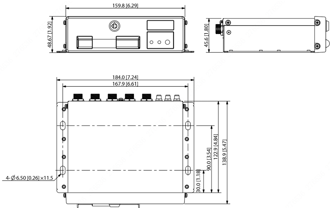
Figure 2-8 Dimension (SSD version) (mm [inch])
