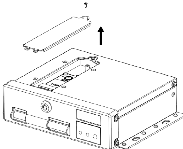
Figure 2-11 Remove box cover
