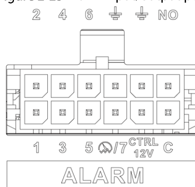
Figure 2-25 Alarm input/output port
