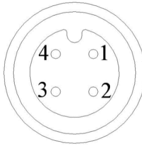
Figure 2-24 Four-cored aviation port
