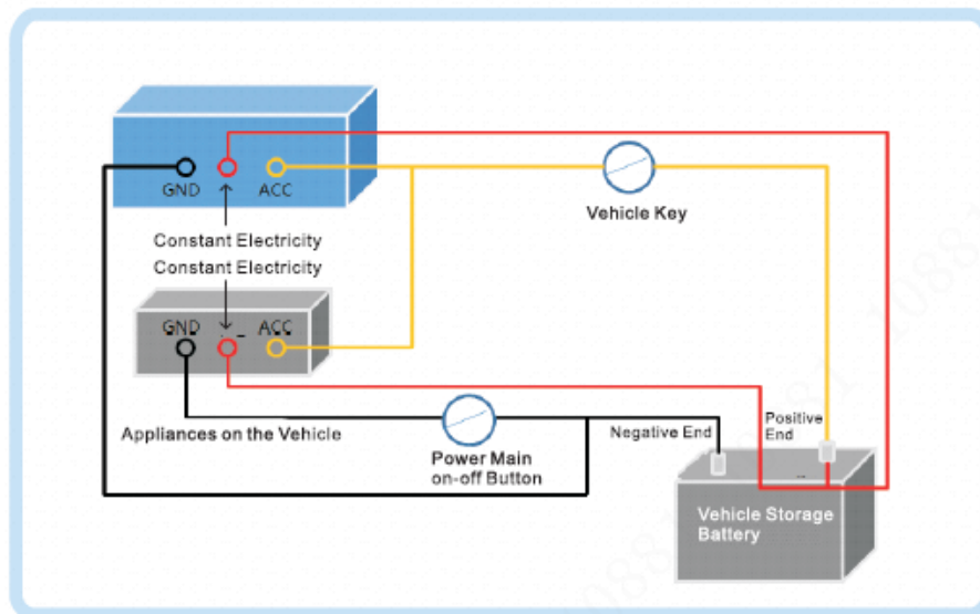
Figure 2-23 Vehicle main switch installed on the negative pole of the vehicle battery
