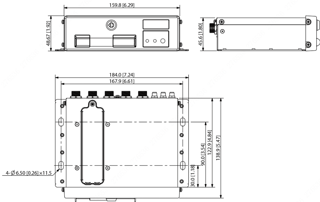
Figure 2-8 Dimension (SSD version) (mm [inch])
