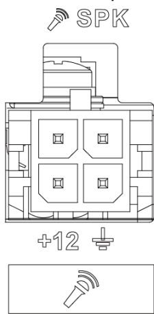
Figure 2-6 External pickup port
