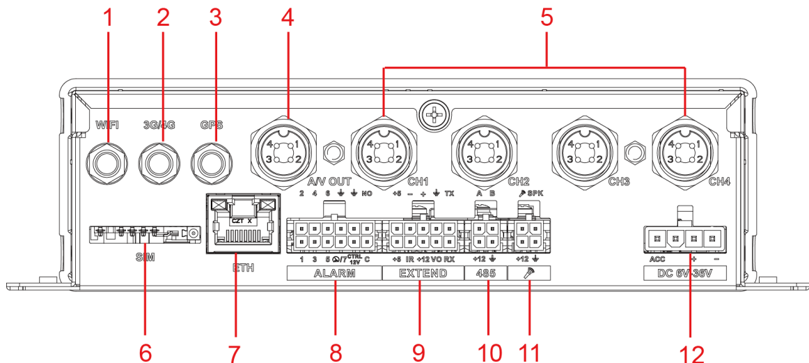
Figure 2-2 Rear Panel
