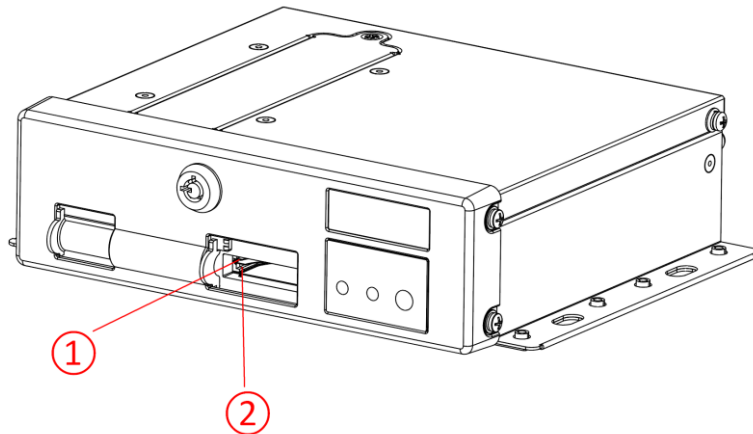
Figure 2-10 Install SD card (SSD version)
