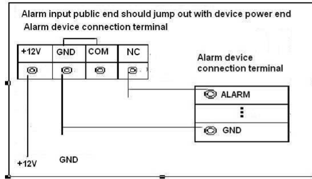
Figure 2-26 Normal Closed alarm input illustration
