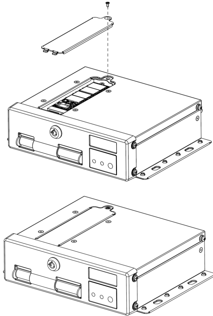
Figure 2-14 Install slot cover
