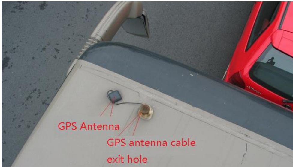
Figure 2-17 Outside Installation
