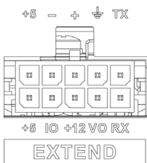
Figure 2-5 EXTEND port
