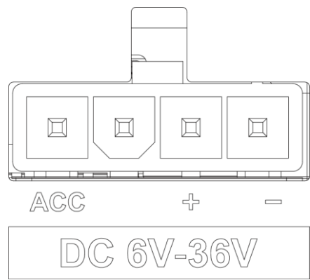
Figure 2-4 Power input interface
