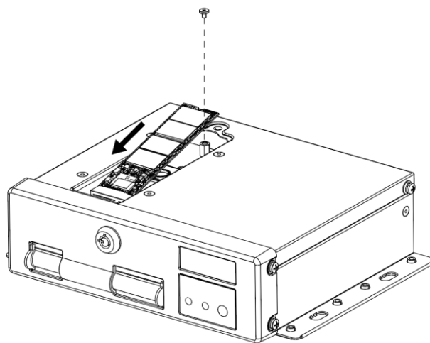
Figure 2-13 Install SSD
