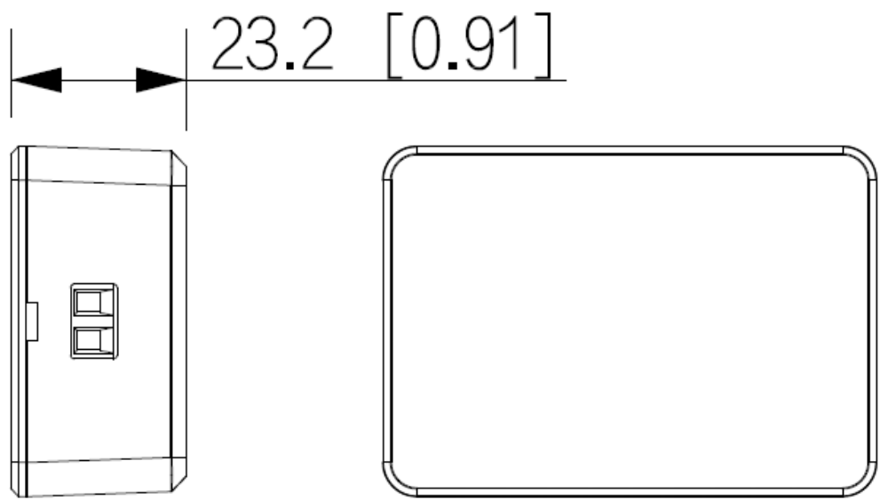
Figure 2-2 Rear panel (unit: mm [inch])
