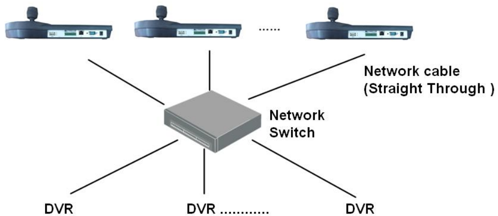
Appendix Figure 2-2 Connection through switch
