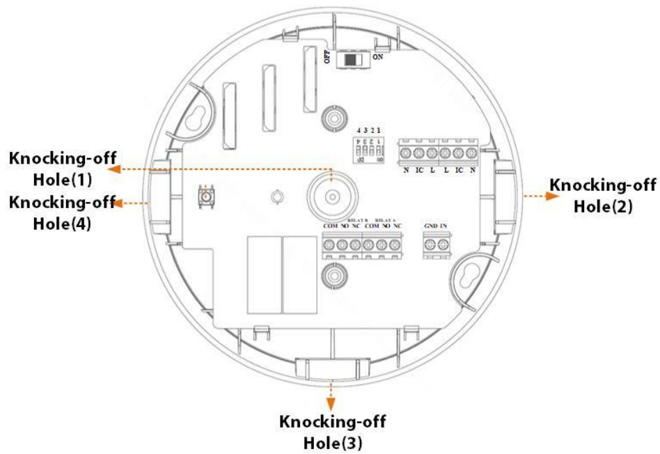
Figure 5-4 Knocking-off holes
