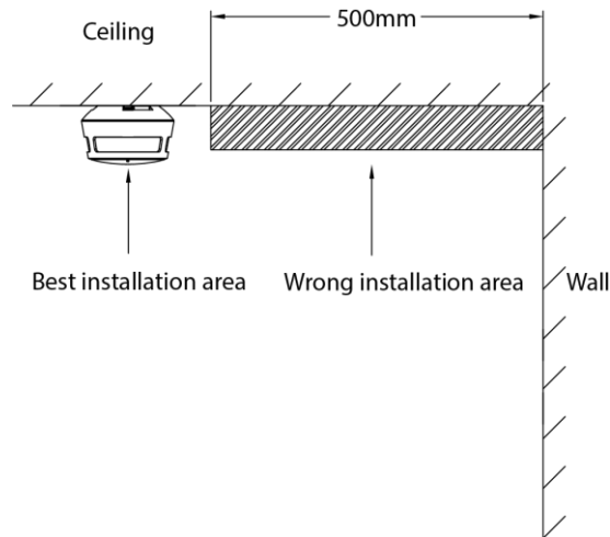
Figure 6-2 Installation position (1)
