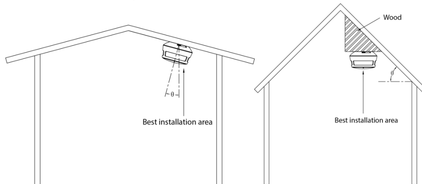
Figure 6-3 Installation position (2)
