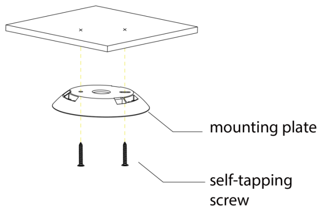
Figure 6-4 Installation step (1)
