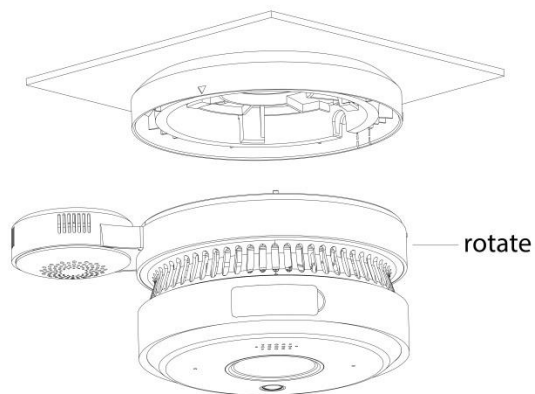
Figure 3-4 Installation (3)
