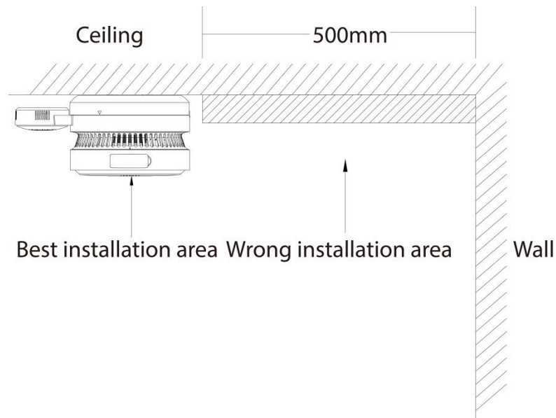
Figure 3-1 Installation position
