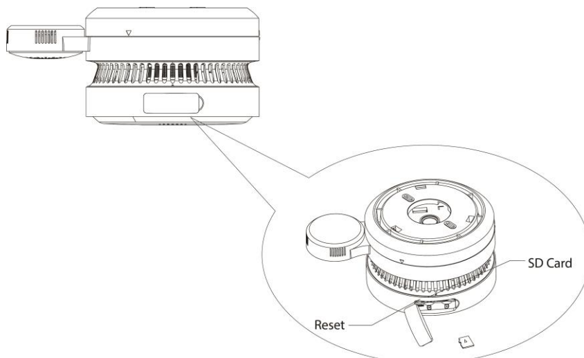
Figure 3-6 SD Card
