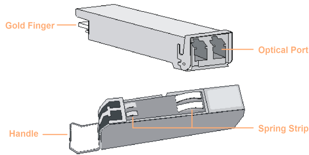
Figure 4-1 SFP module structure
