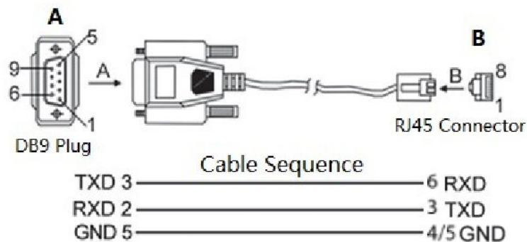
Figure 4-6 Cable sequence of RJ45 DB9
