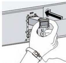
Figure 4-2 SFP module installation
