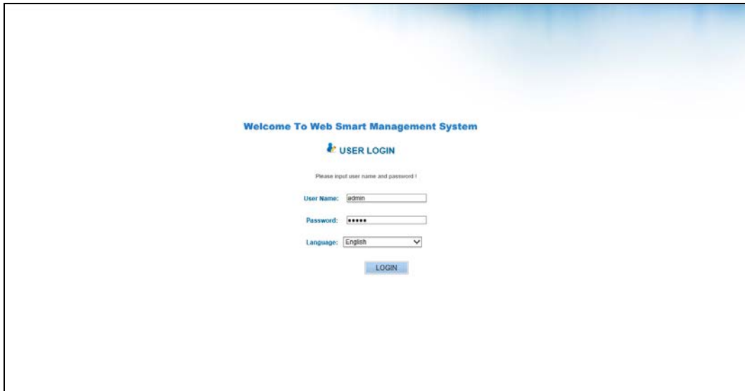
Figure 7- Login Windows
