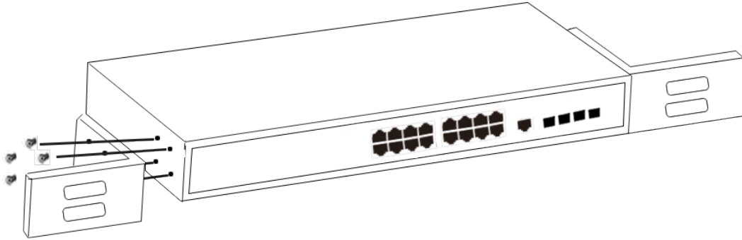
Figure 3 - Bracket Installation
