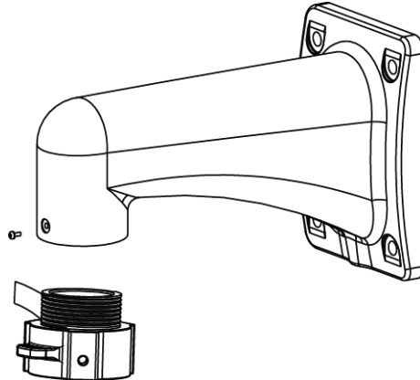
Figure 3-3 Screw the quick connector
