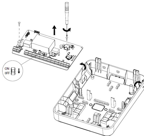
Figure 4-2 Main board
