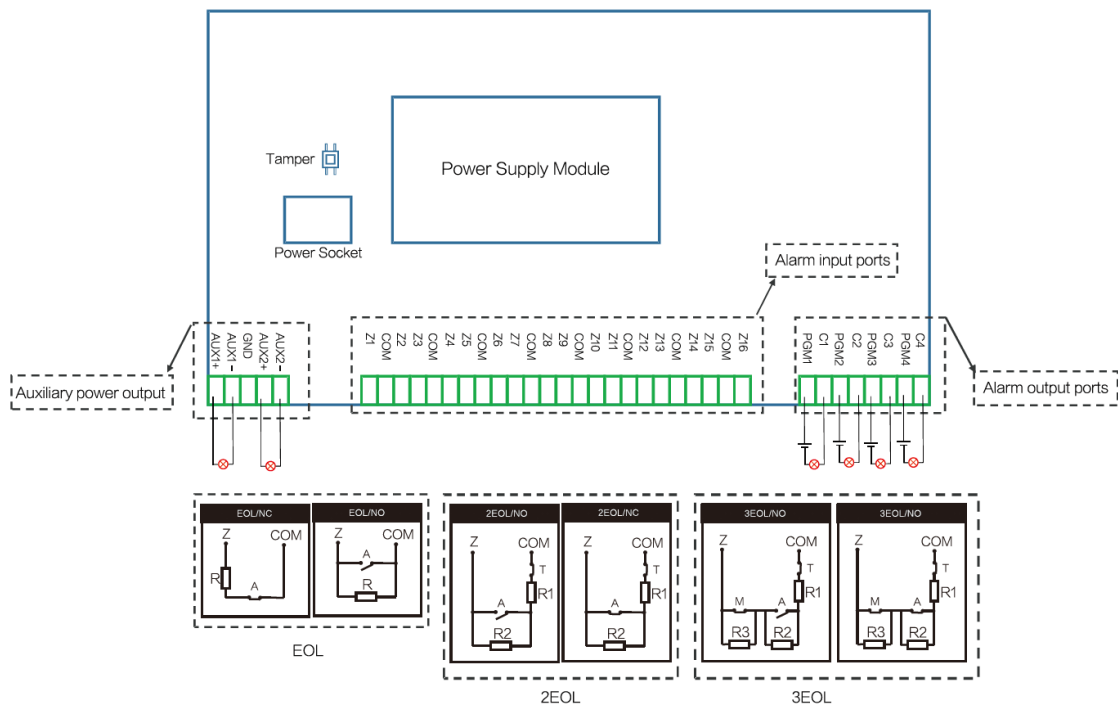
Figure 6-1 Alarm input cable connection
