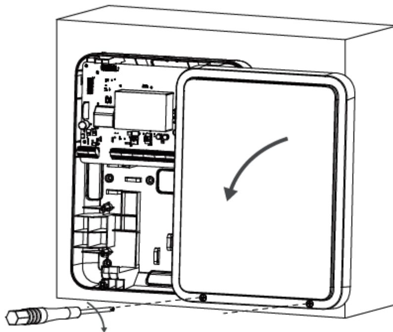
Figure 5-4 Install (3)
