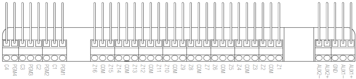
Figure 5-3 Wiring diagram
