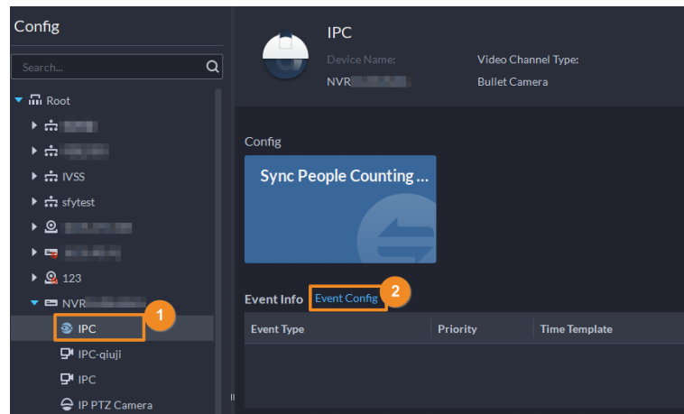
Figure 3-32 Go to the event configuration (channel)
