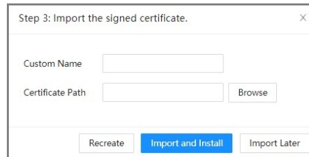
Figure 16-10 Import a CA certificate
