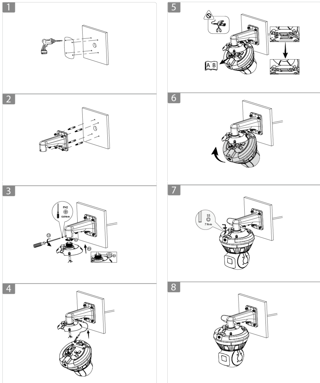
Figure 4-3 Wall mount
