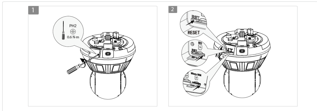
Figure 4-2 Install the SD/SIM card
