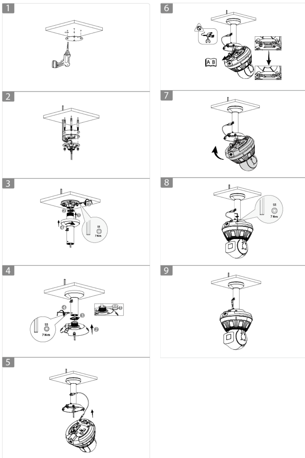
Figure 4-4 Ceiling mount
