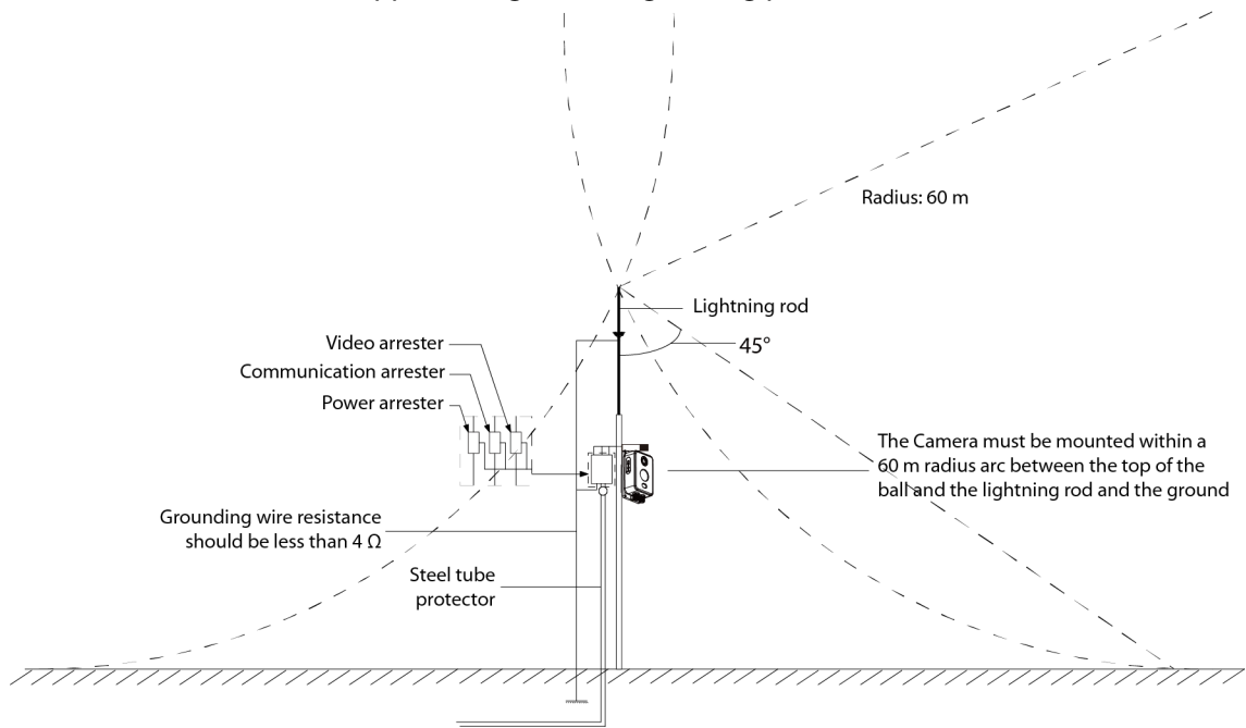
Appendix Figure 1-1 Lightning protection
