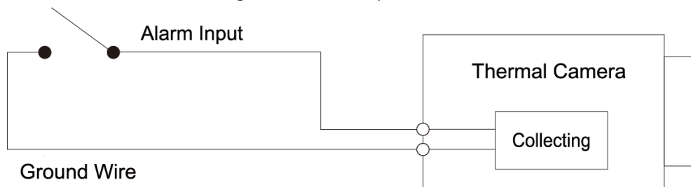
Figure 5-1 Alarm input
